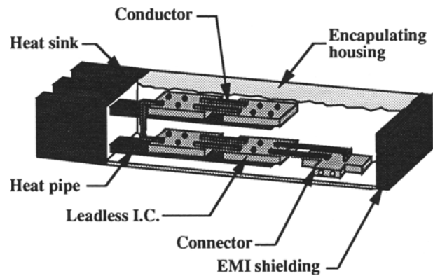
Figure 9 Integrated electronic/mechanical package.
