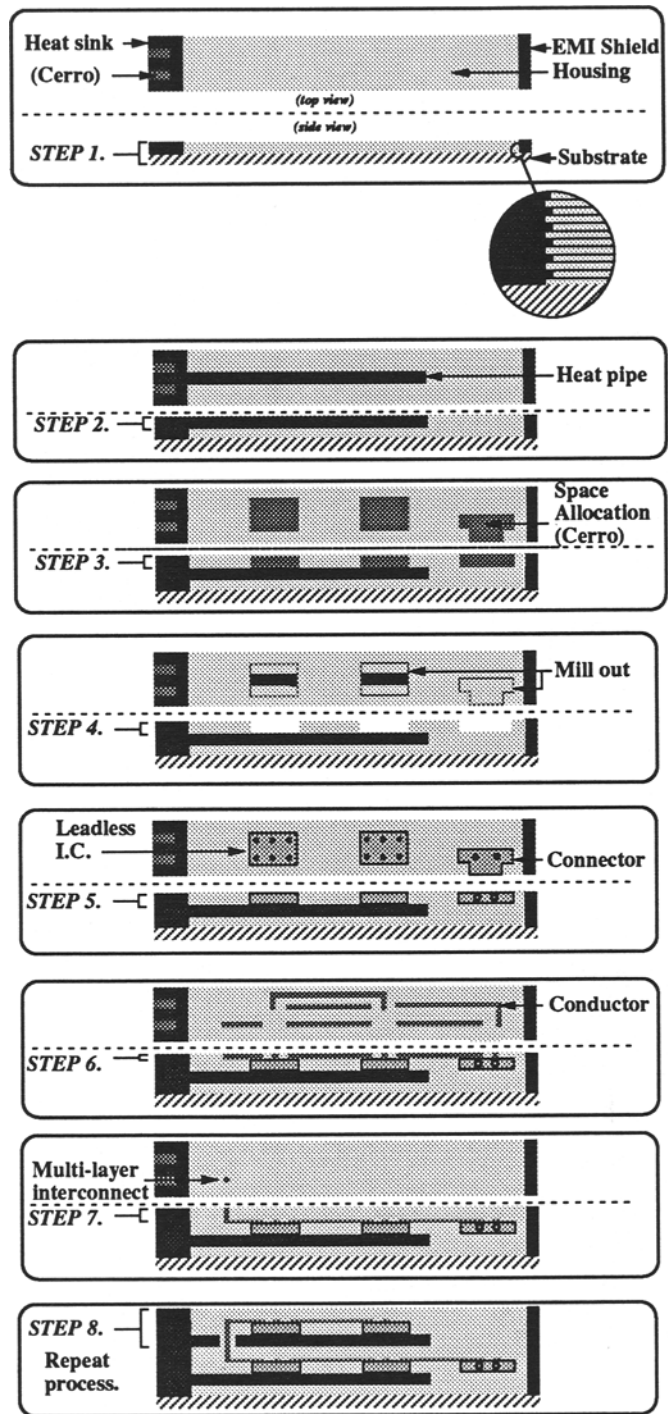
Figure 11 Fabrication steps.
