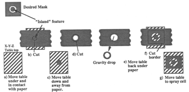
Figure 7 Mask cutting sequence.
